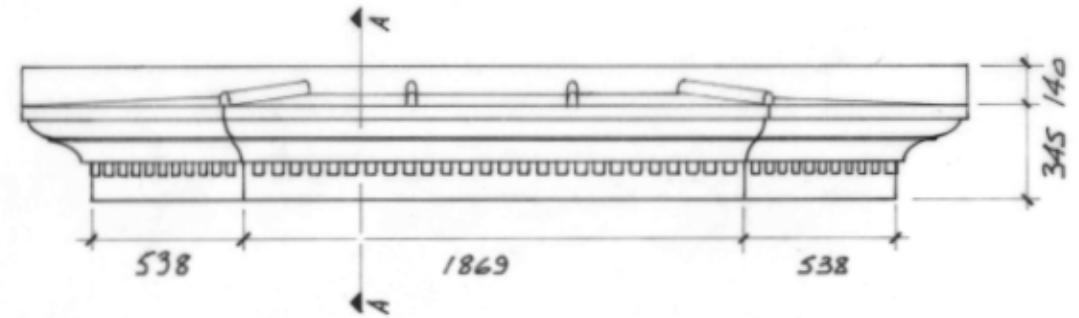
FRONT ELEVATION 1:20
