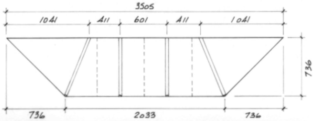
ROOF PLAN 1:20
