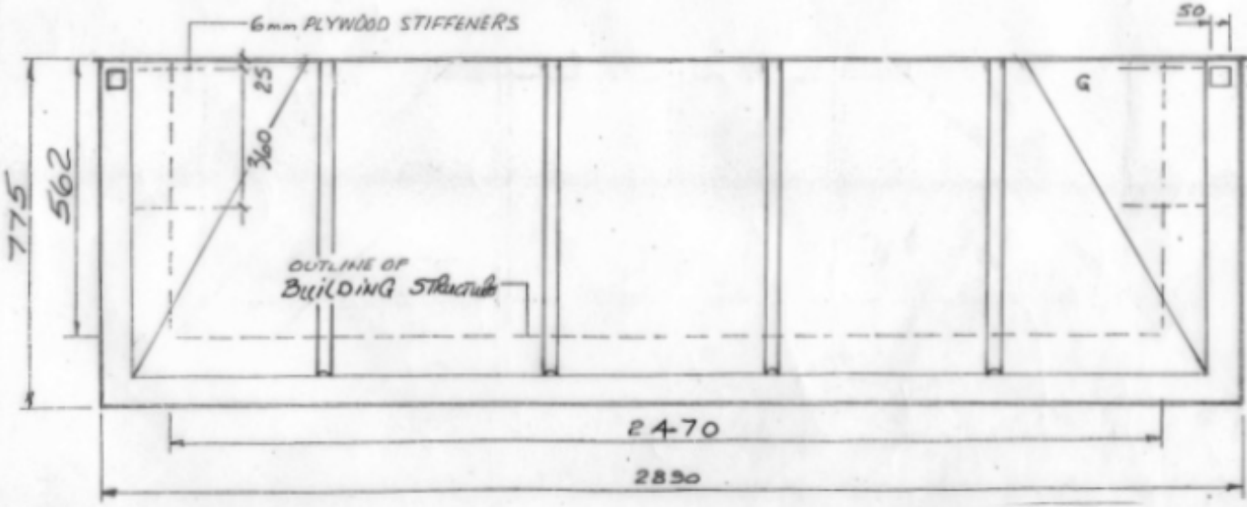
ROOF PLAN NT3
