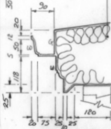
FASCIA DETAIL
