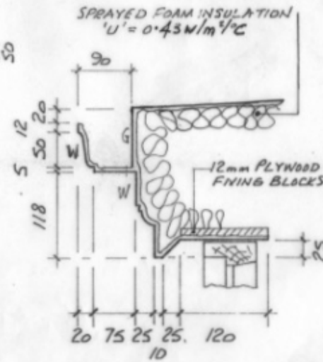
FASCIA DETAIL 1:5
