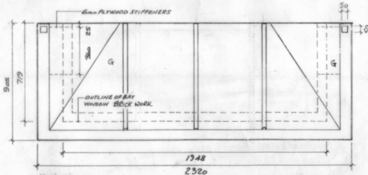
ROOF PLAN 10:125
