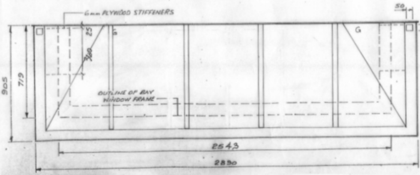
ROOF PLAN Note: Colour = G = Grey, W = WHITE
