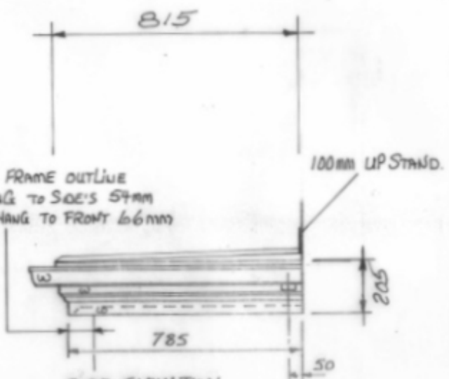
SIDE ELEVATION
