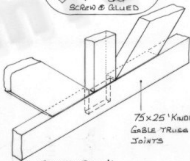
TRUSS DETAIL
