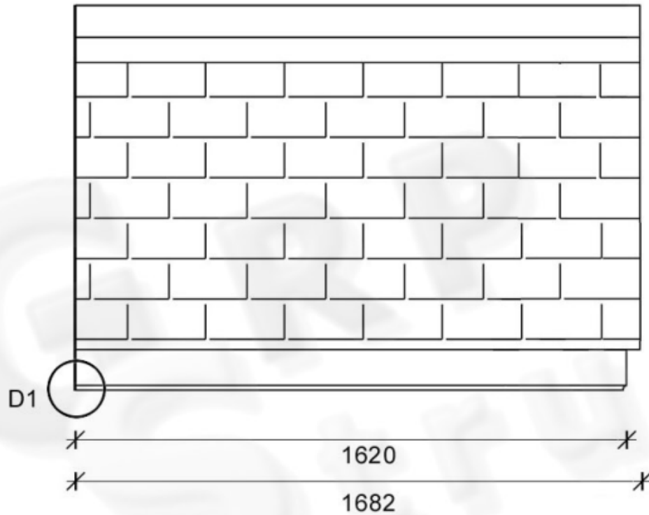
FRONT ELEVATION
