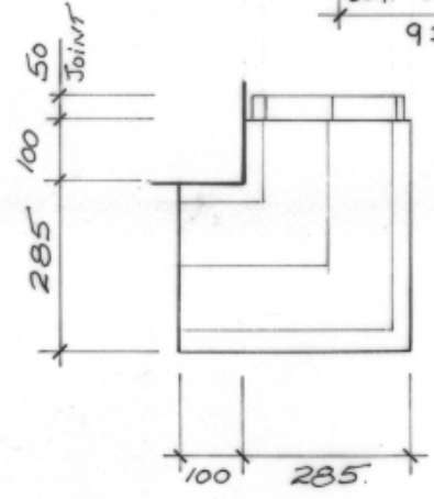
CORNER DETAIL
