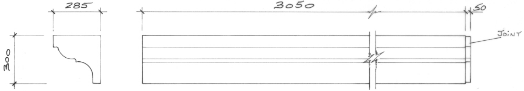
ELEVATION 1:10
