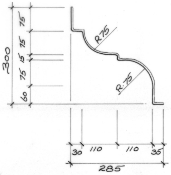
TYPICAL SECTION.
