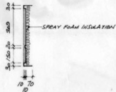
SECTION THROUGH INFILL PANEL SPOKES SMOOTH FINISH PANELS LIGHT RENDERED FINISH
