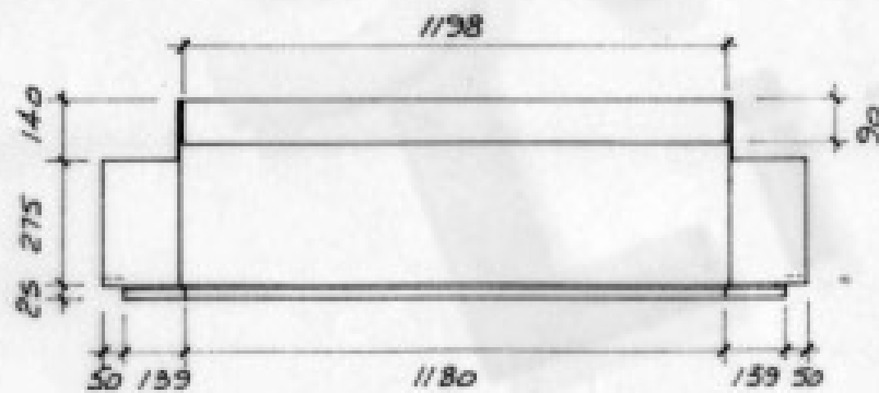
REFLECTED SOFFIT PLAN
