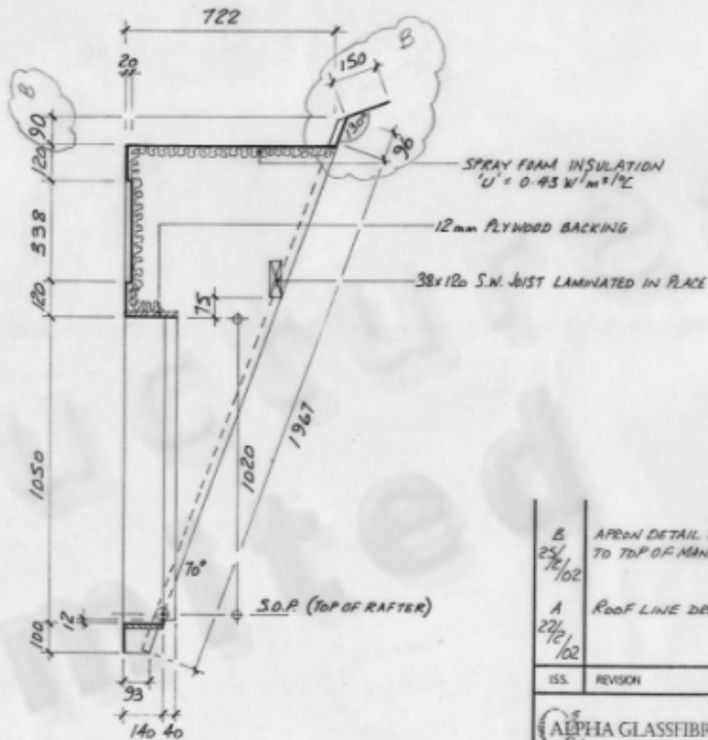
SECTION THROUGH E 1:12.5
