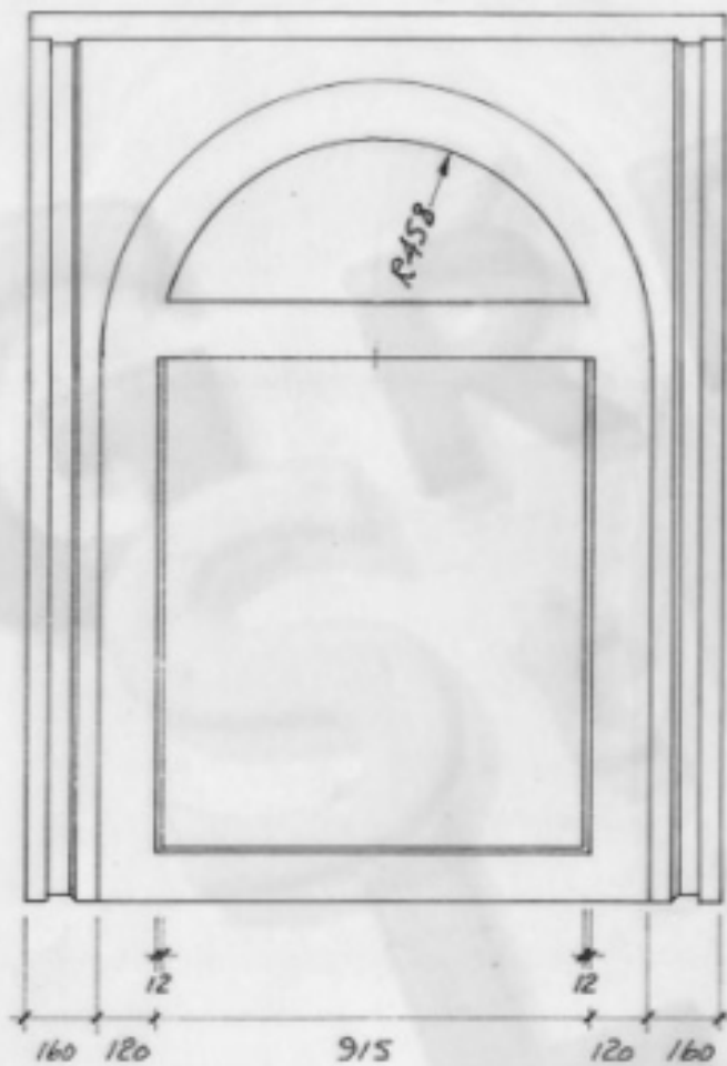
FRONT ELEVATION 1:12.5
