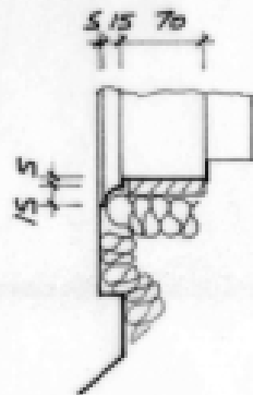
CILL DETAIL 1/5
