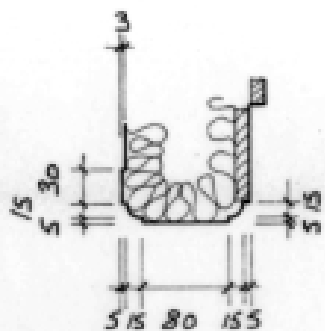
CORNER 'POST' DETAIL 1/5
