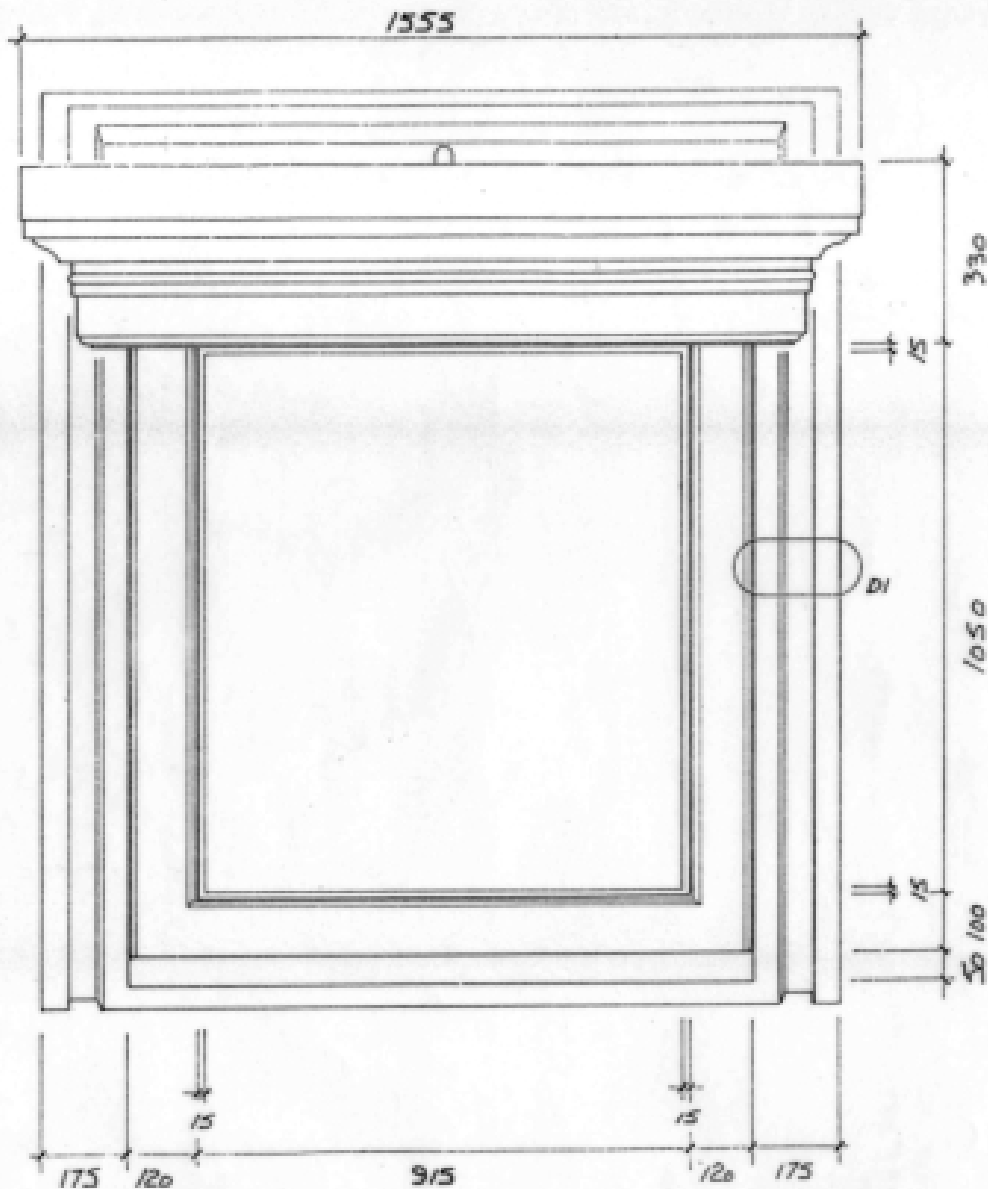
FRONT ELEVATION 1/10
