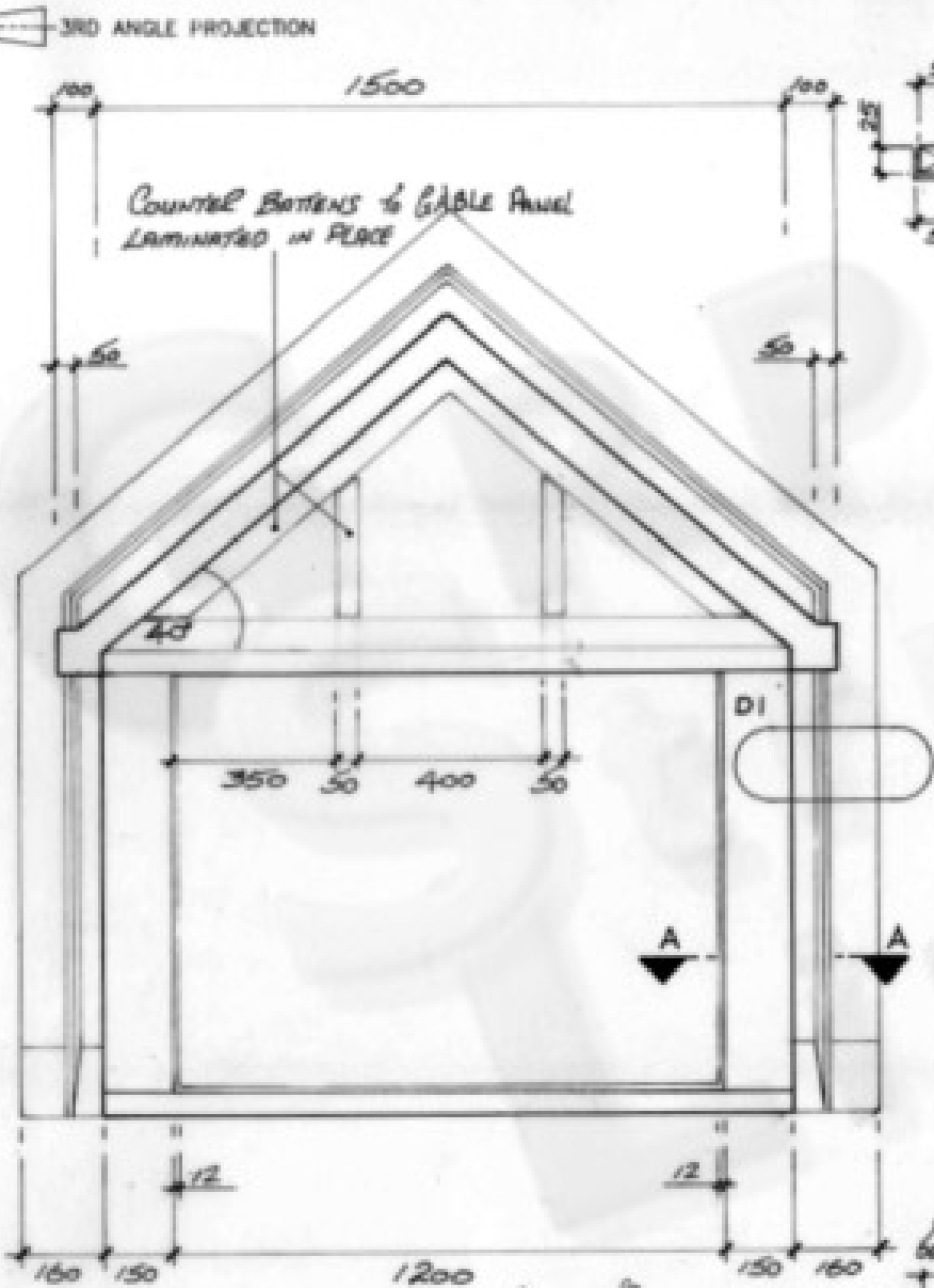
FRONT ELEVATION
