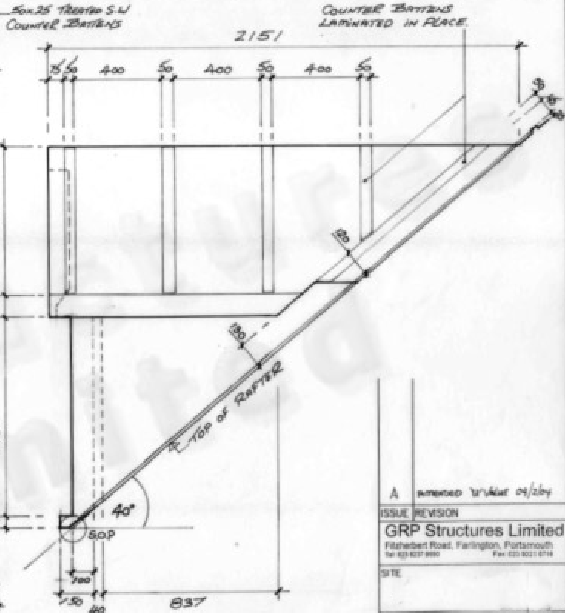
SIDE ELEVATION
