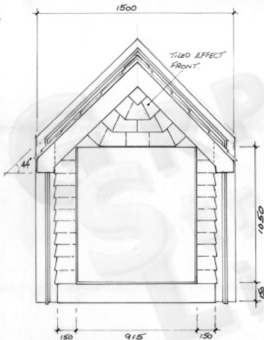
FRONT ELEVATION
