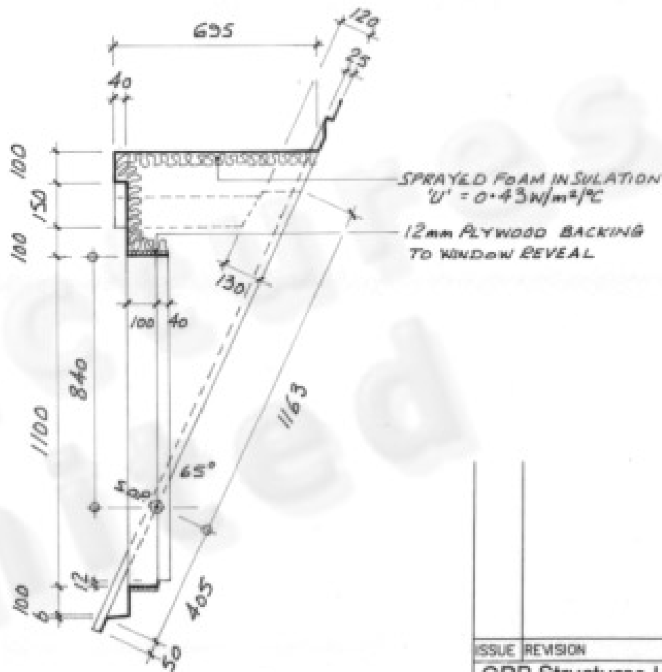
SECTION THROUGH
